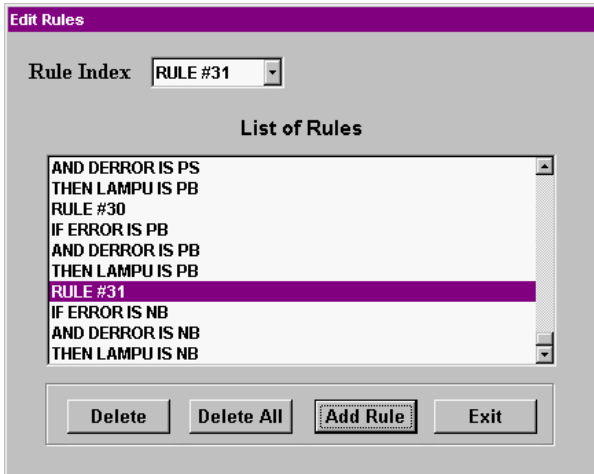
Gambar 6 Menu Edit Rule
