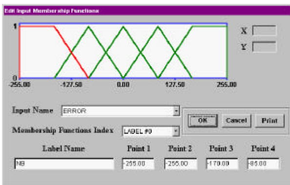
Gambar 4 Menu Input Membership Function
